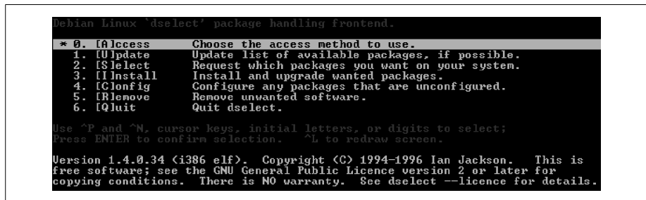
Figure 40-1. The dselect screen
